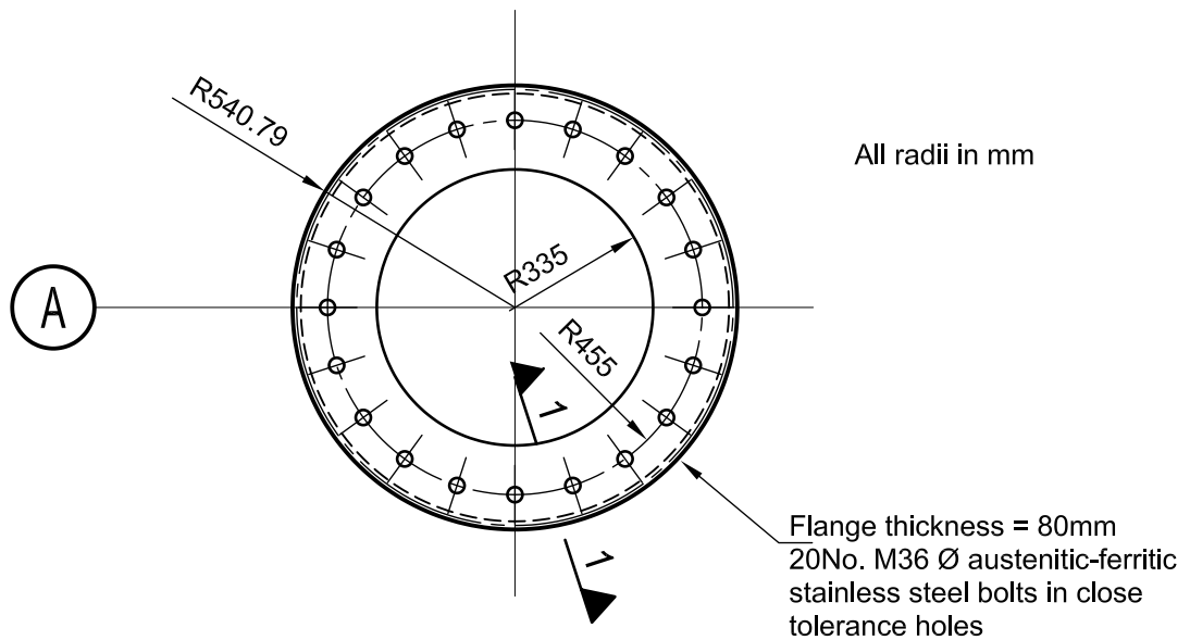
Plan of Flange at 85.606m OD Level (Scale 1:20)
