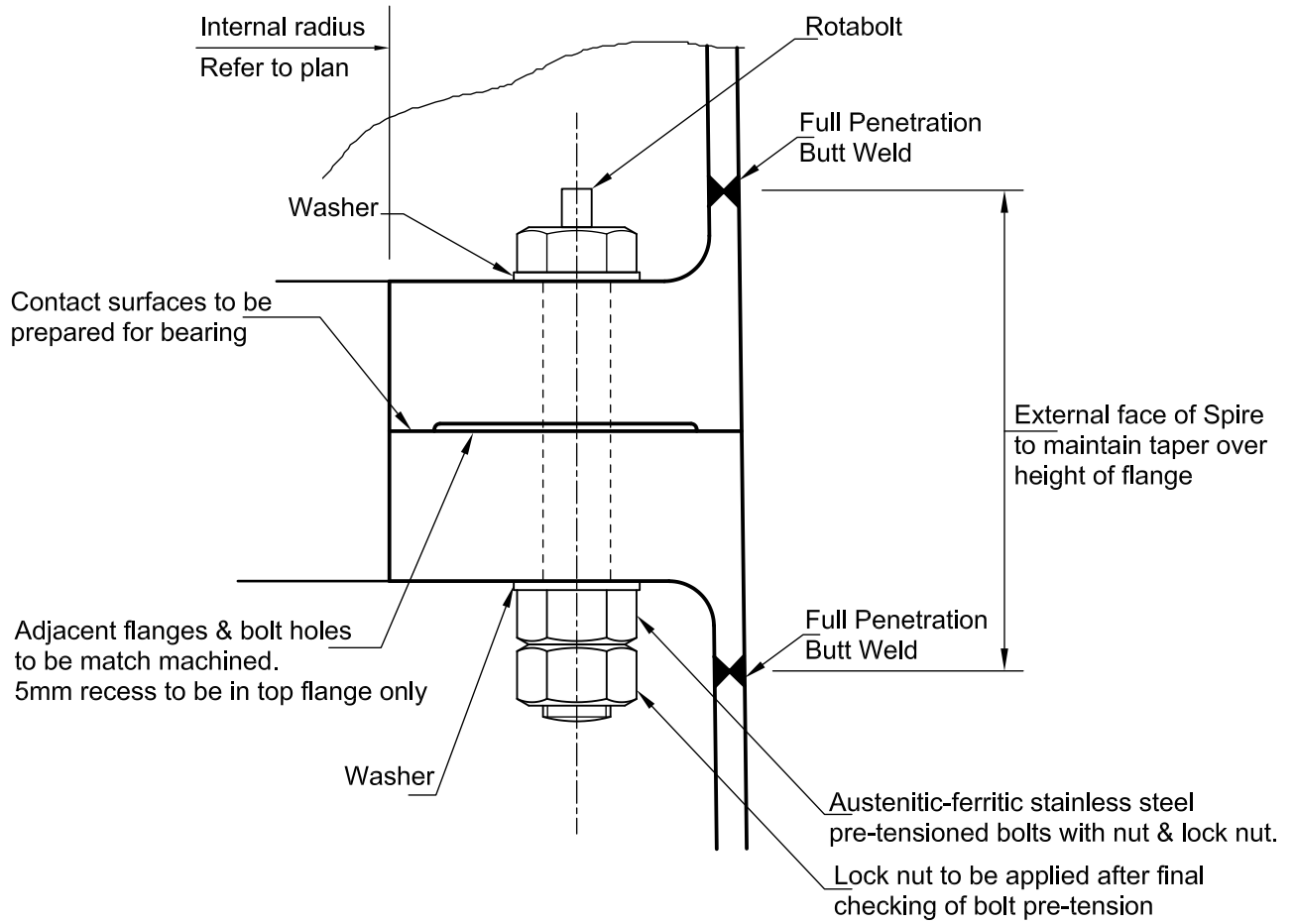
Section 1 - 1 (Scale 1:10)
