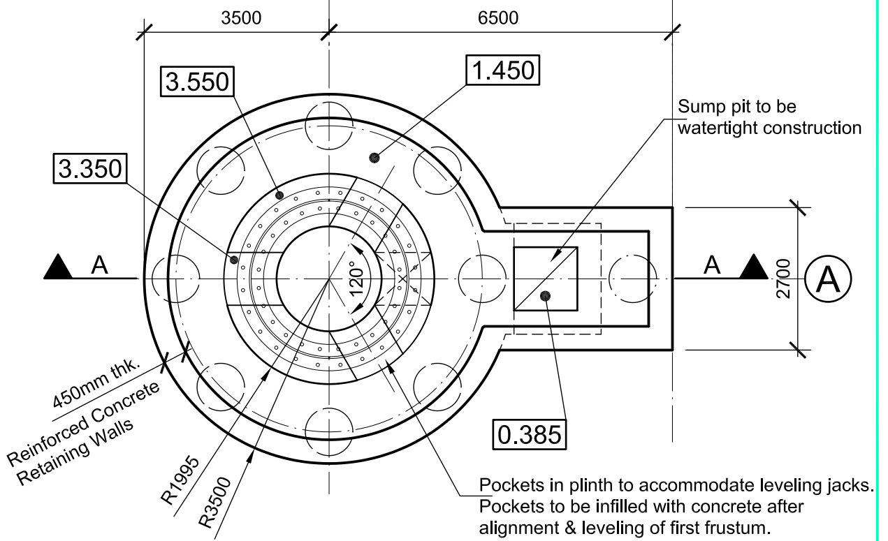
Plan on Base (Scale 1:100)
