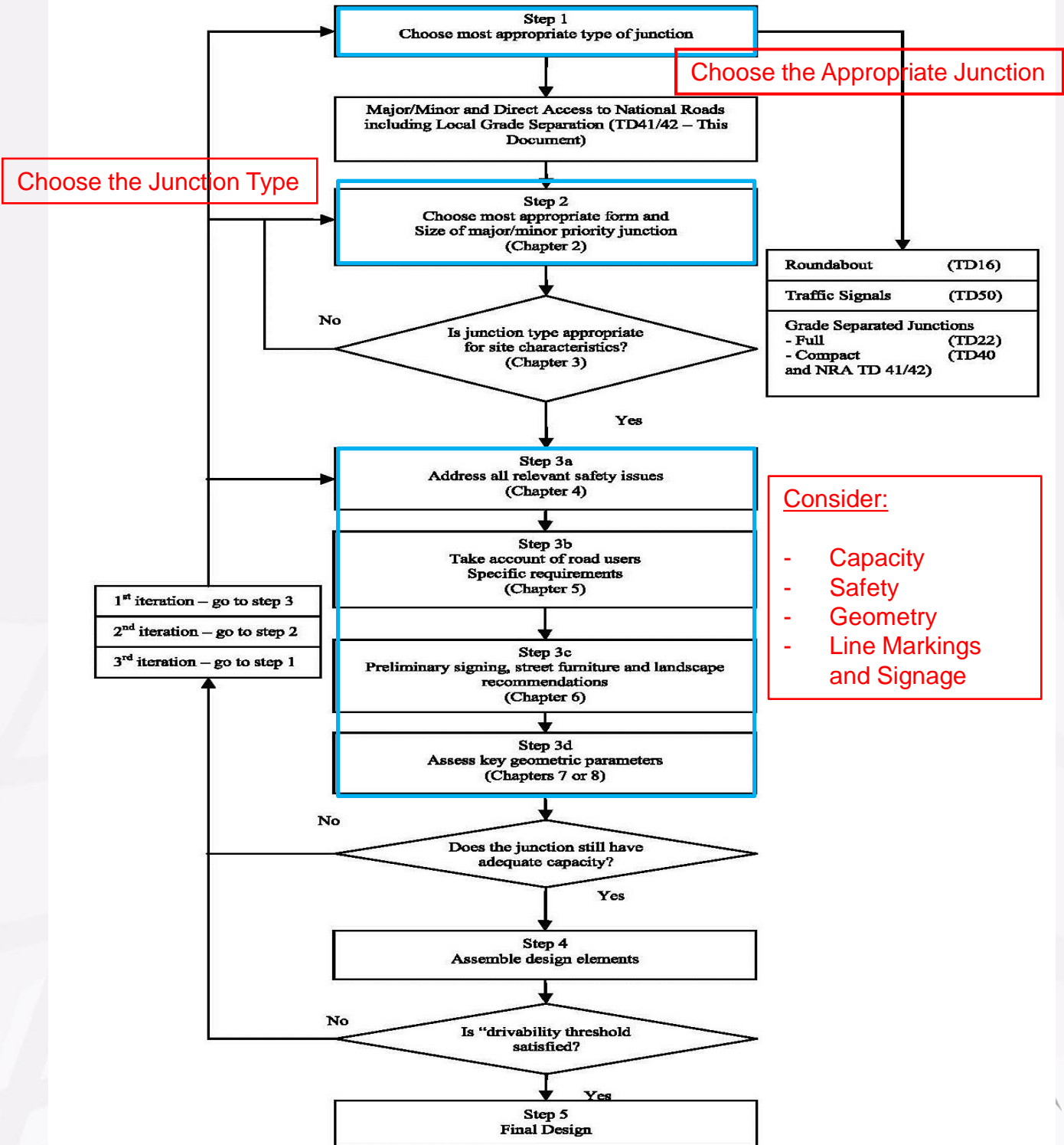
Figure 2/1: Flow Chart Outlining Design Procedure (Para 2.12 to 2.18)
